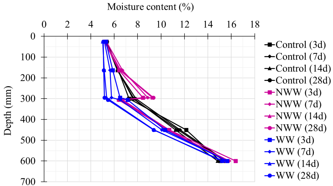
Figure 4.7 Gravimetric moisture content profile for silty sand with 5% fines with and without the geotextile at different waiting periods.
