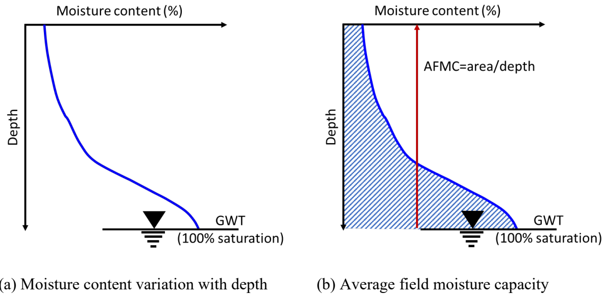
Figure 3.3 Profile of field moisture content (capacity) with depth in soil.
