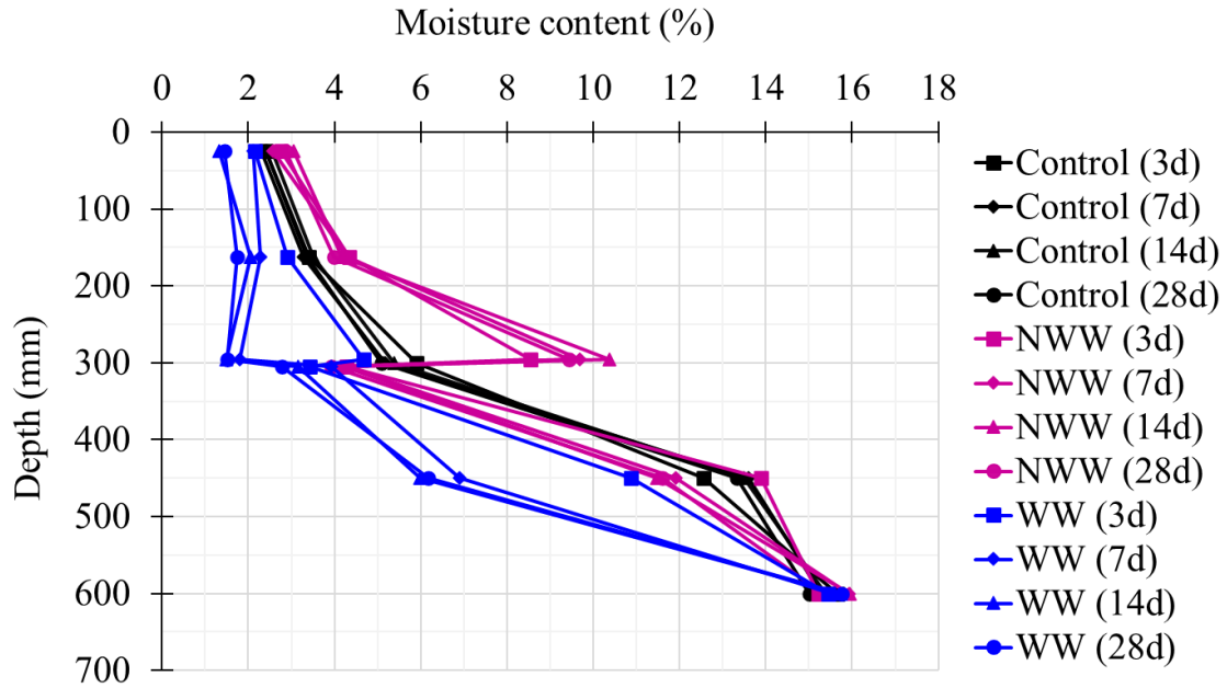
Figure 4.6 Gravimetric moisture content profiles for the sand with 0% fines with and without the geotextile at different waiting periods.
